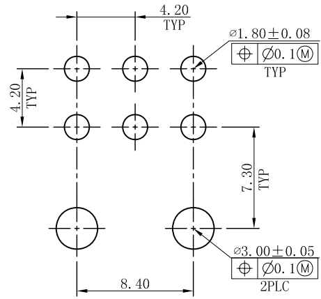
RECOMMENDED P. C. B. HOLE LAYOUT (TOLERANCE: ± 0.05)
