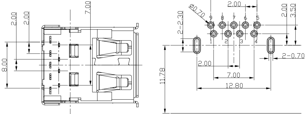
RECOMMENDED PCBA LAYOUT (TOLERANCE±0.05)
