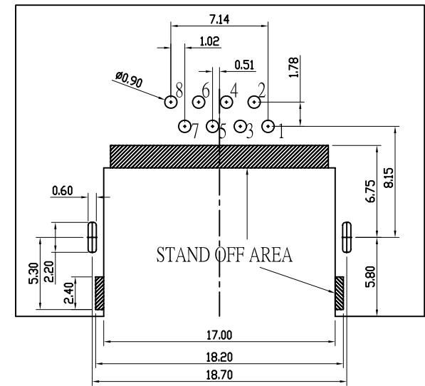
PCB LAYOUT TOP VIEW TOL:±0.05(THICKNESS=1.60)
