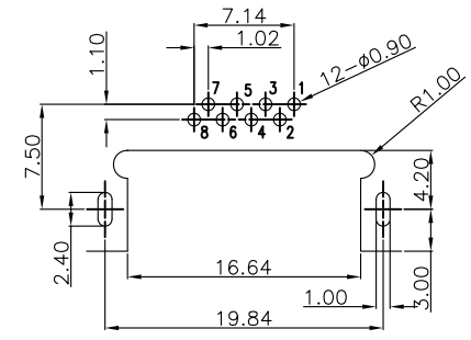
PCBLAYOUT TOL:±0.05
