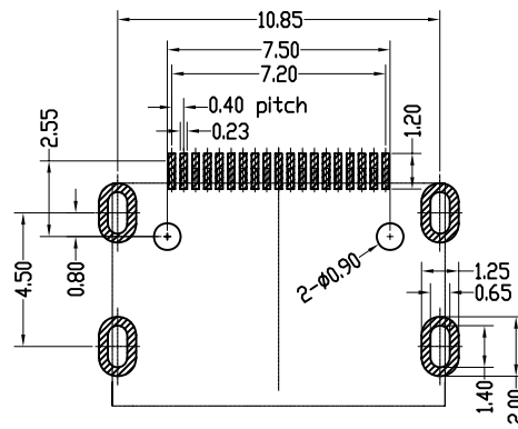
RECOMMEND PCB LAYOUT PCB TOLERANCE:±0.05
