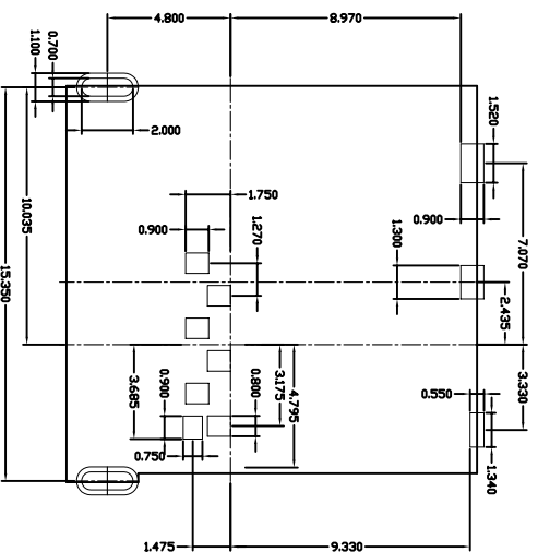
RECOMMENDED PCB LAYOUT TOL:(±0.05)
